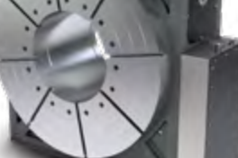
HRT1000 4-AXIS • 1,000 mm Platter • 35°/sec • Resolution 0.001° • HRT800 also available
