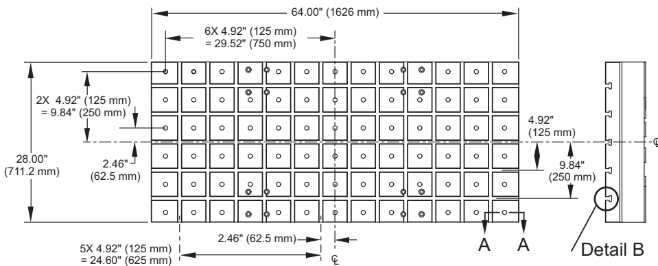
VM-6 Inch Table Dimensions
