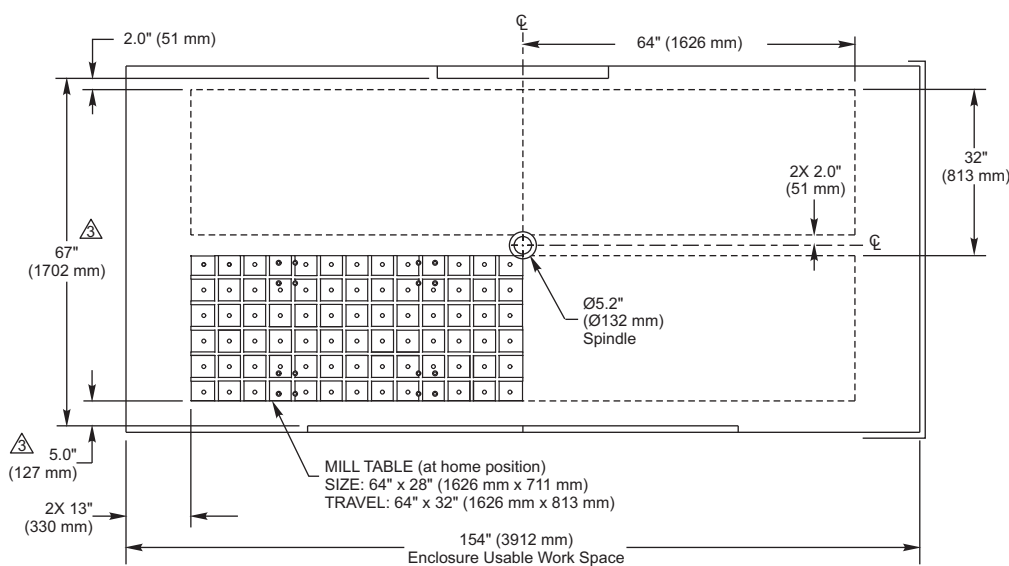
Detail B Inch and Metric
