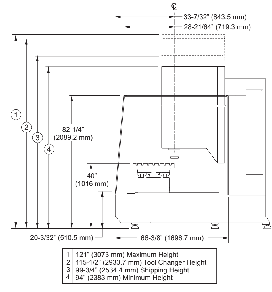
VM-3 Sheet Metal Removed for Clarity
