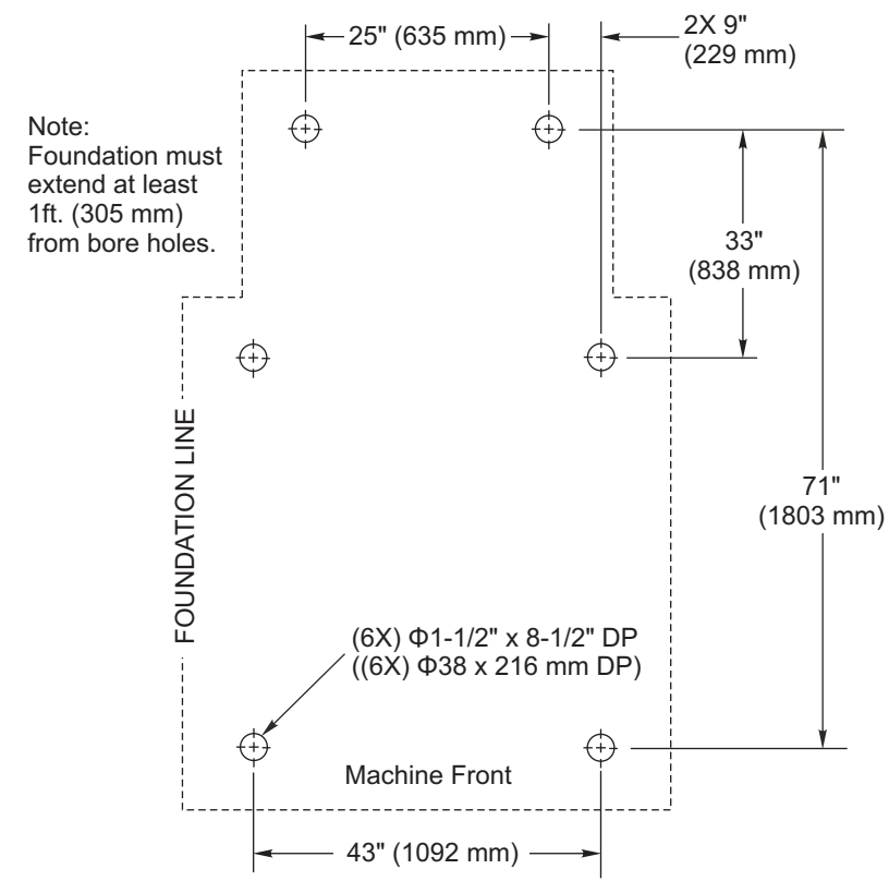
VM-3 Anchor Pattern
