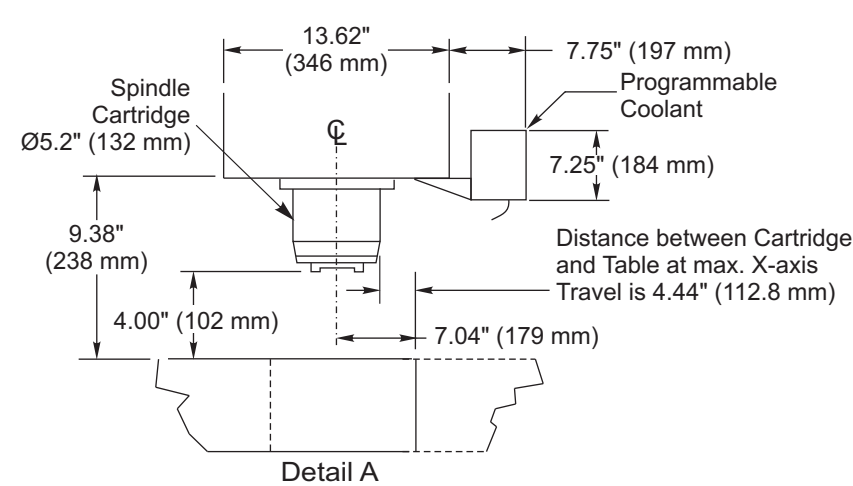
VM-3 Enclosure Usable Work Space
