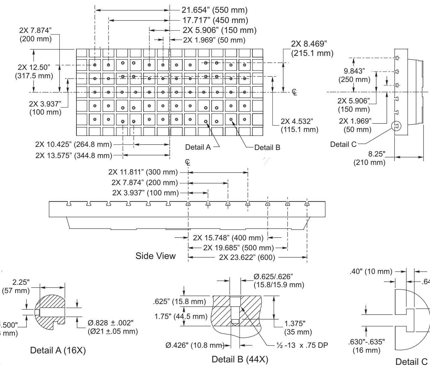
VM-3 Table Dimensions
