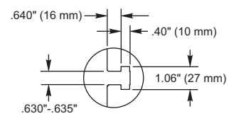
Detail B (7X)
