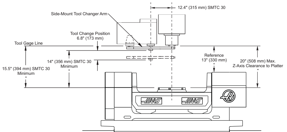
FRONT VIEW
