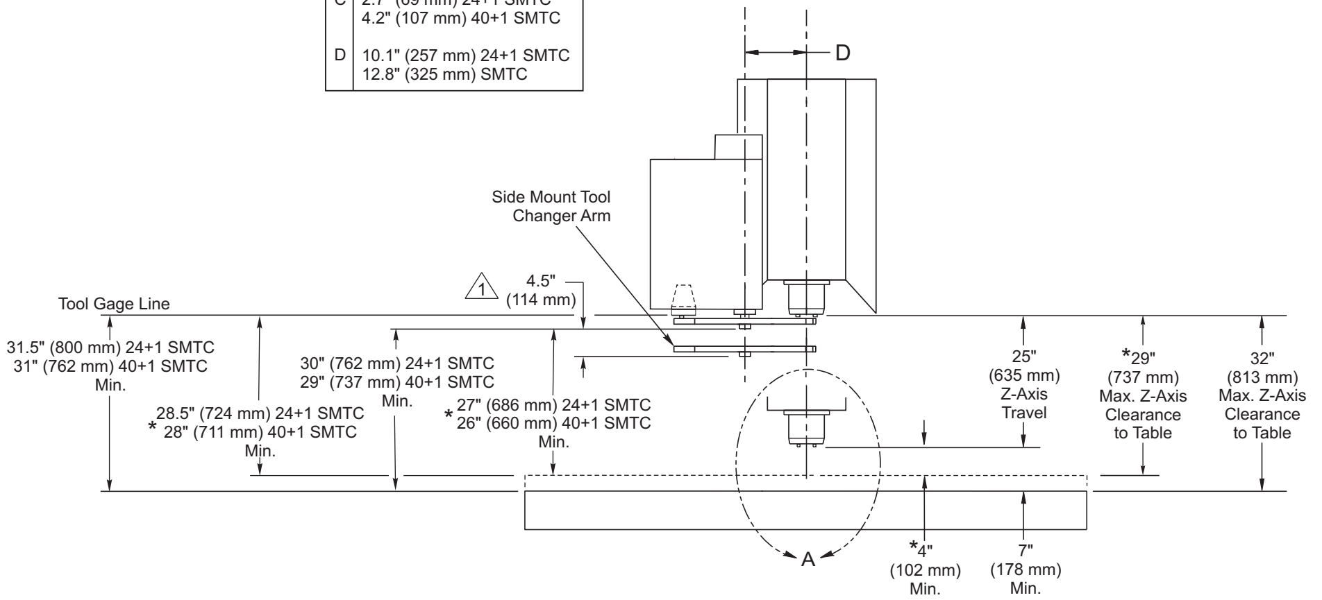
40 Taper 24+1 Side Mount Tool Changer 40 Taper 40+1 Side Mount Tool Changer Double Arm Work Envelope
