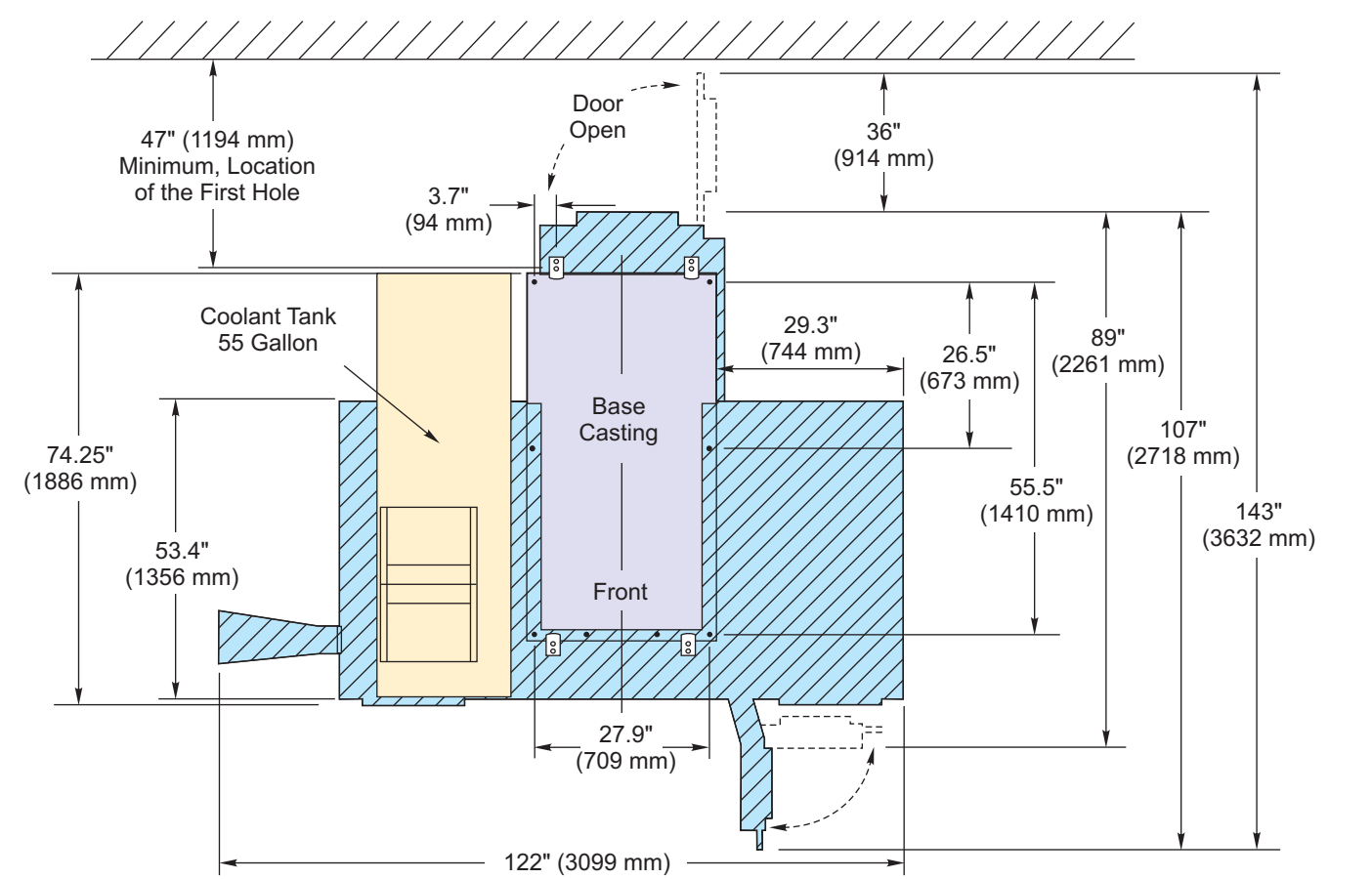
*Coolant Tank Dimensions 55 Gallon (208.2L): 84.4" (2143 mm) X 27.5" (699 mm)
