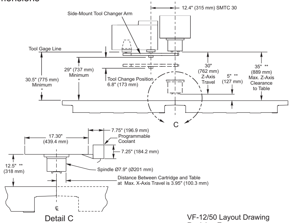
VF-12/50 Enclosure Usable Work Space
