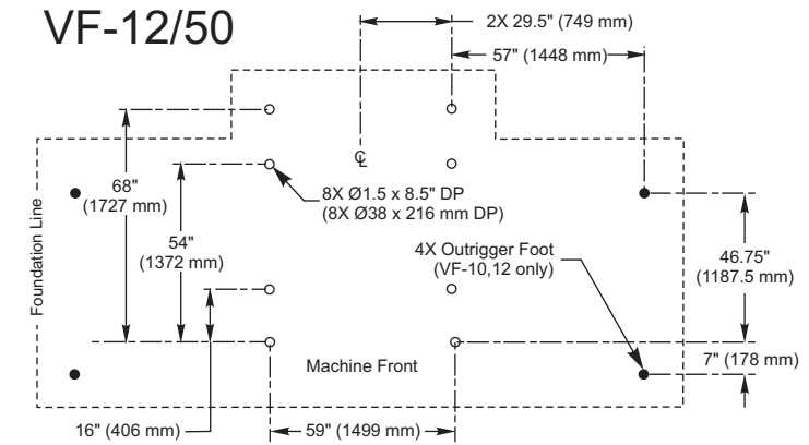
VF-12 Anchor Pattern
