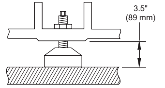
Leveling Pad Pin Dimension
