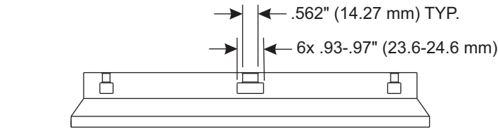
TR310 Platter Dimensions
