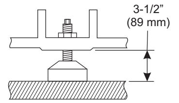
4X Leveling Pad Pin Dimension
