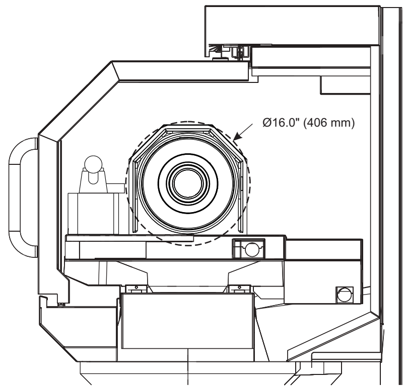
Max turning diameter with 3/4" (20 mm) tool post
