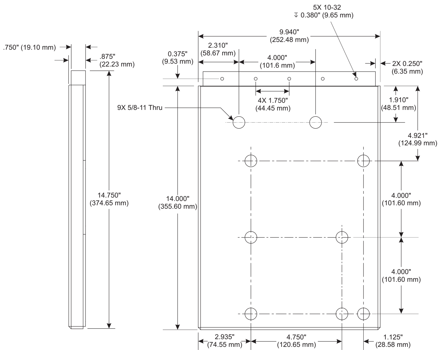
TL-2 Cross Slide Dimensions
