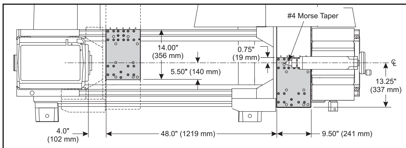
TL-2 Enclosure Work Space (Top View)
