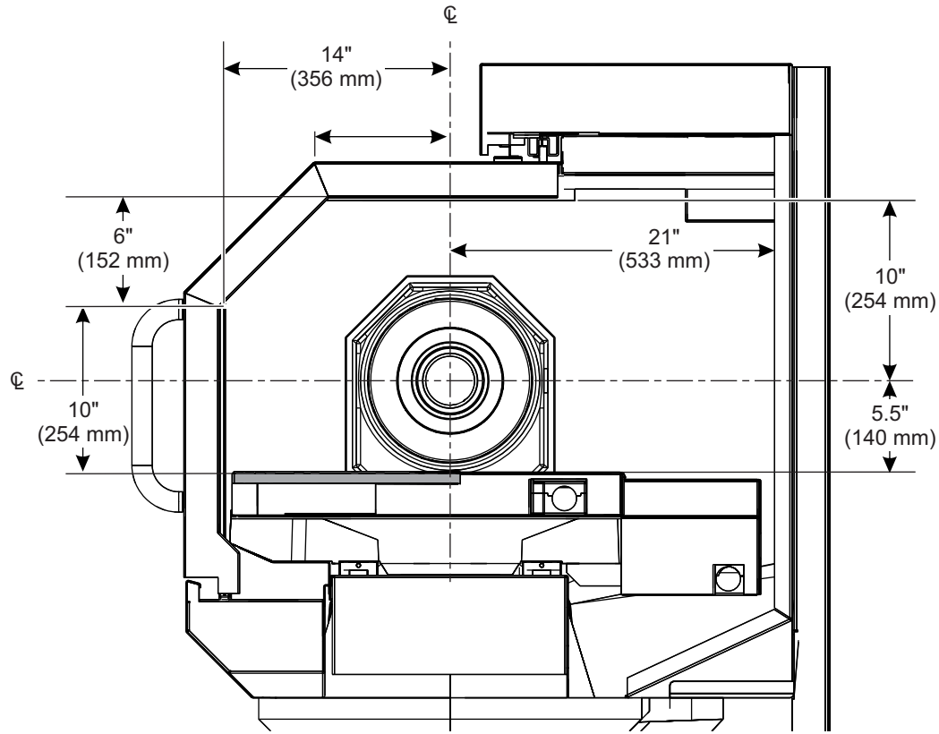
TL-2 Enclosure Work Space (Right Side)
