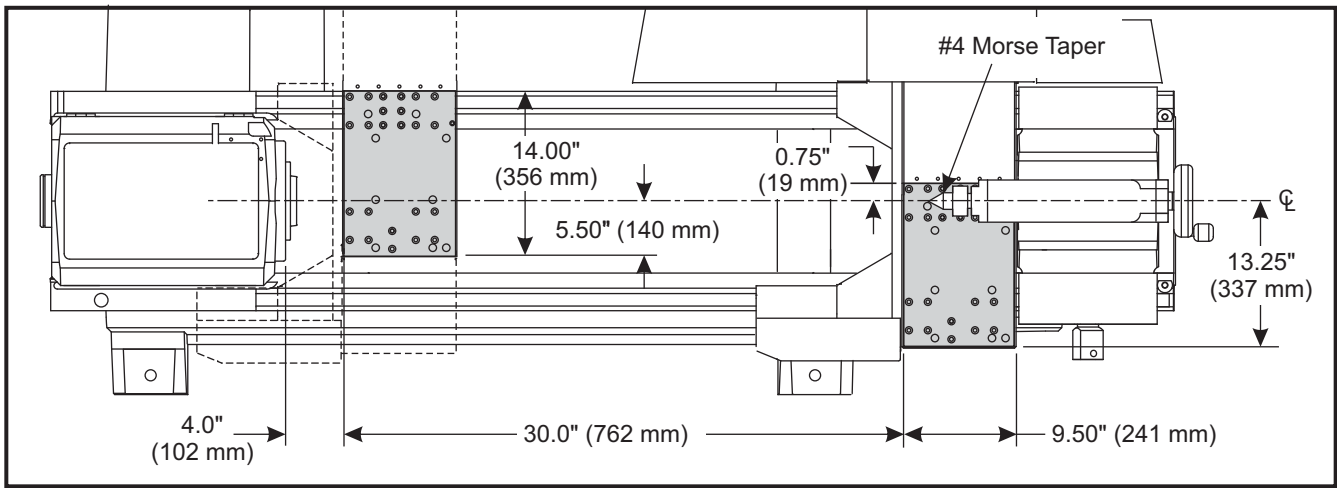
TL-1 Enclosure Work Space (Top View)
