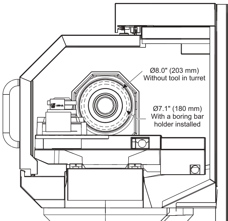
Max turning diameter with 4-station automatic tool turret
