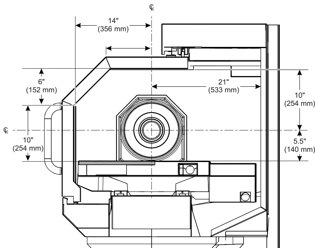
TL-1 Enclosure Work Space (Right Side)
