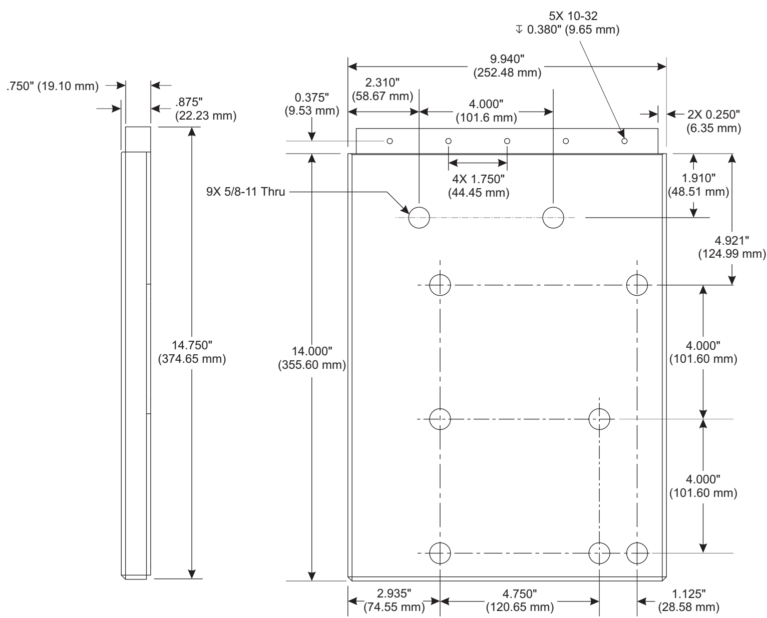
TL-1 Cross Slide Dimensions
