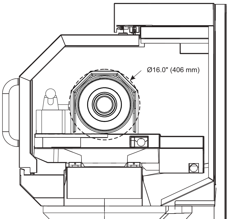
Max turning diameter with 3/4" (20 mm) tool post
