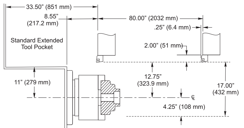
Axis Travels - ST-40L/45L with Standard BOT
