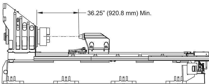
ST-40L/45L Tailstock and Steady Rest Travel #5 Morse Taper
